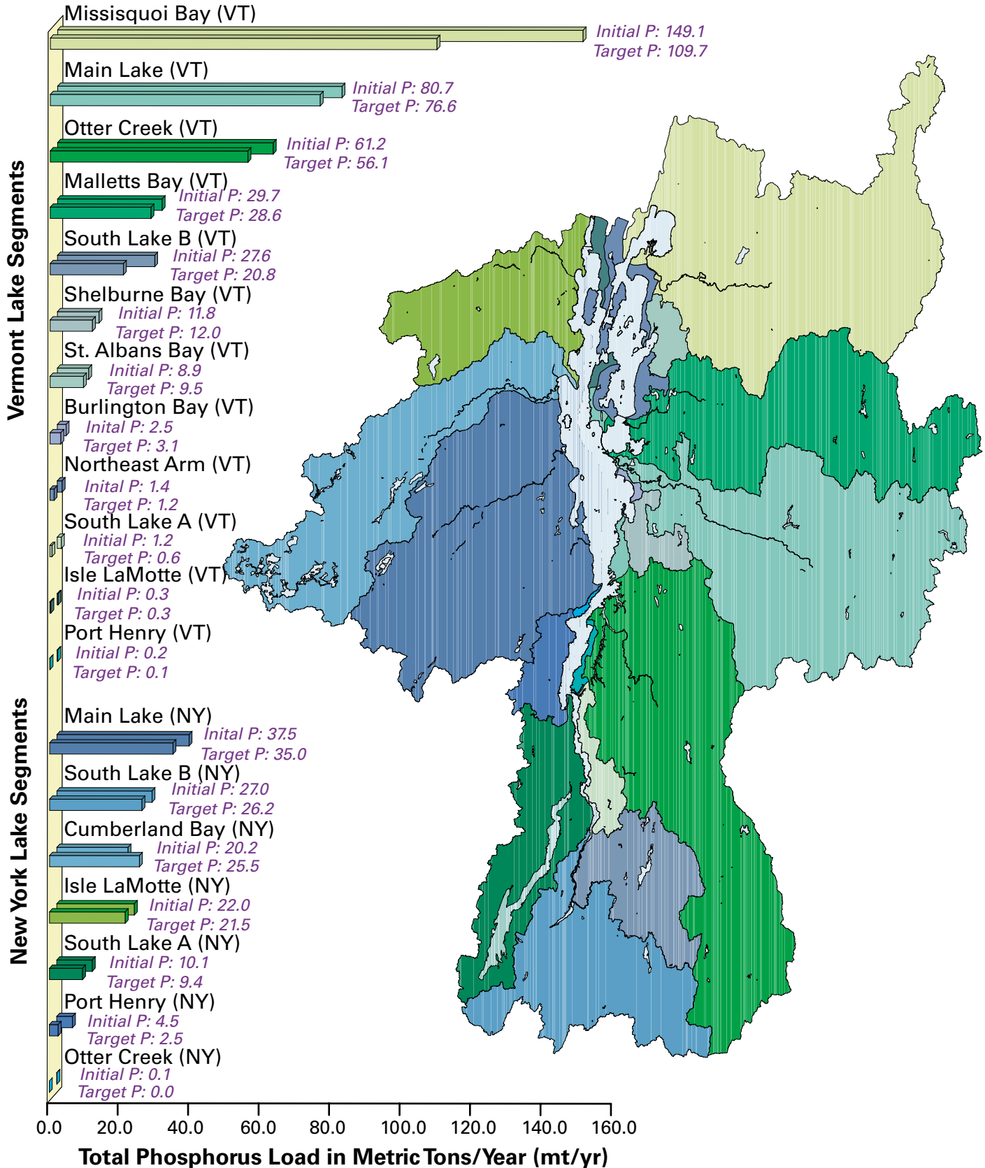
Initial (1995) and Target Phosphorus Loads by Lake Segment Showing Adjacent Watersheds in Metric Tons/Year (mt/yr)
